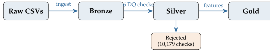
Figure 1: Bronze → Silver → Gold pipeline with rejected-records store.
